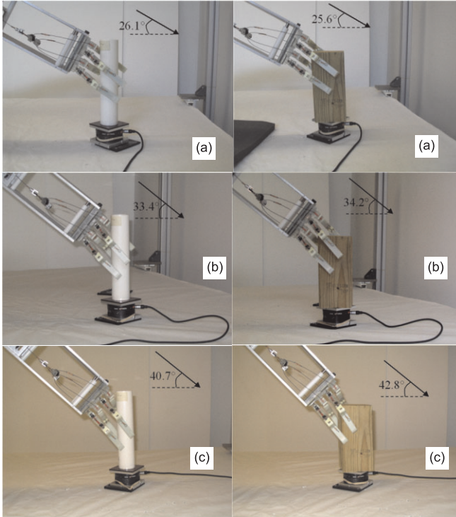
Fig. 9. Two target objects (PVC cylinder with radius 24 mm and wood block with square cross-section 90 mm side length) at three locations ((a), (b), and (c)). Note the differences in approach angle for the locations, the main factor affecting the force and grasp space results.
